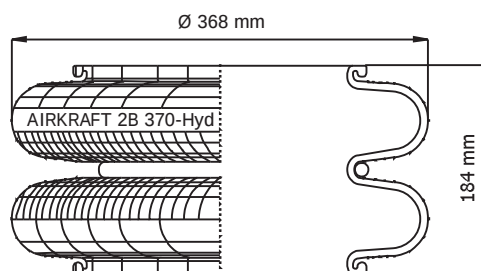
Bellows 4 Ply
