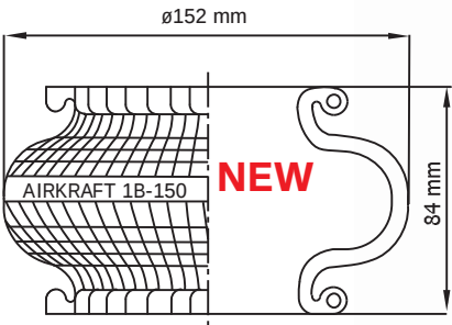
Bellows 2 Ply
