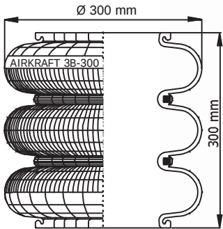
Bellows 2 Ply
