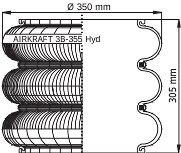
Bellows 4 Ply
