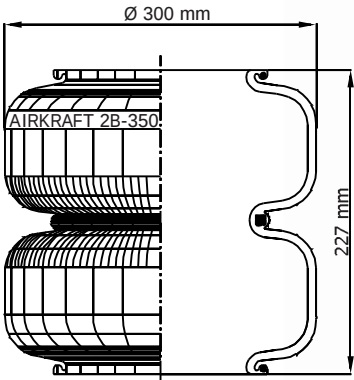
Bellows 2 Ply
