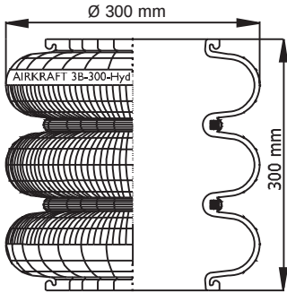
Bellows 4 Ply
