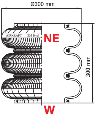
Bellows 3 Ply
