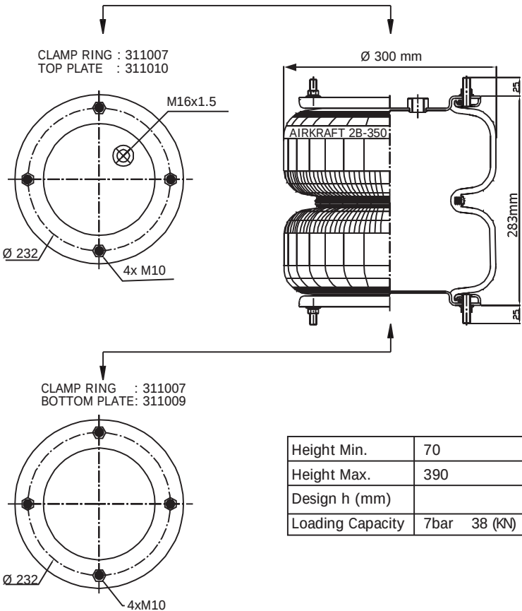
Bellows 2 Ply
