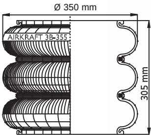
Bellows 2 Ply
